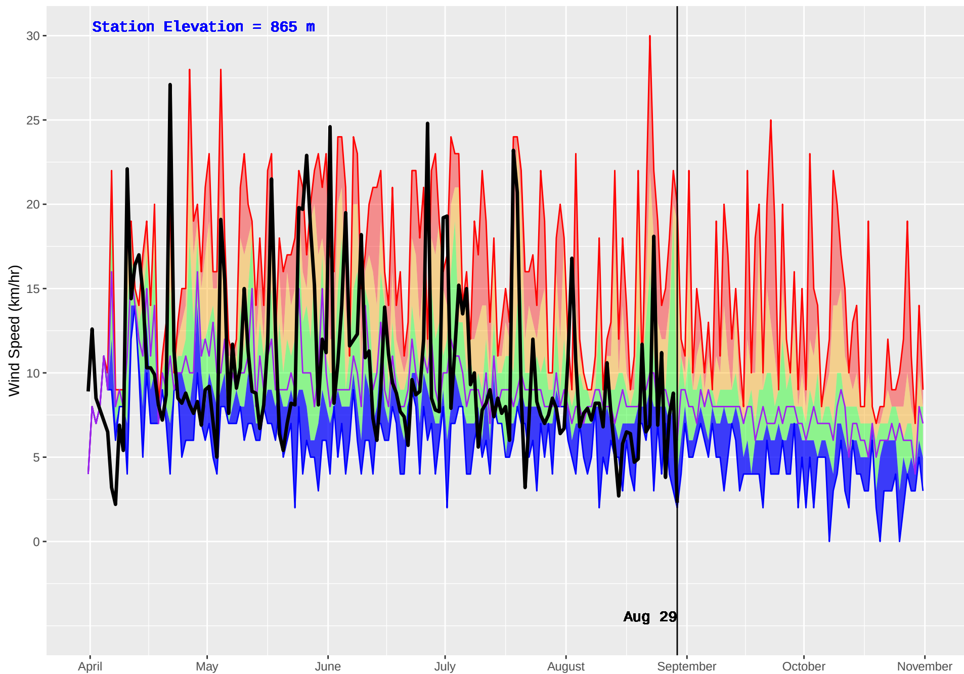
FIVE MILE (1029) : Historical (2008–2016) and Current (2018) Daily Wind Speed
